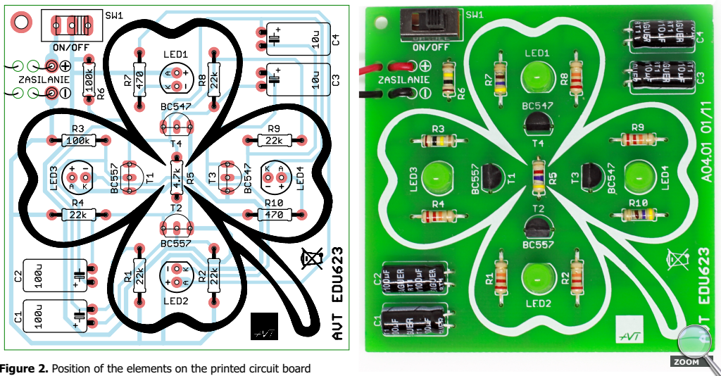
Figure 2. Position of the elements on the printed circuit board
