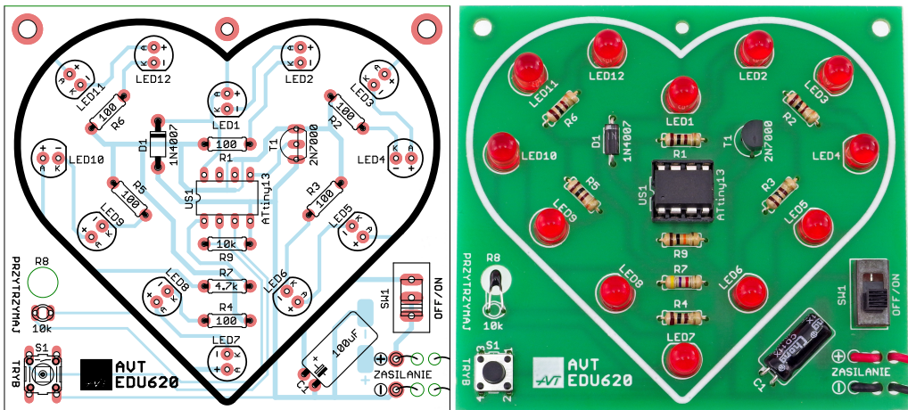
Figure 2. Position of the elements on the printed circuit board
