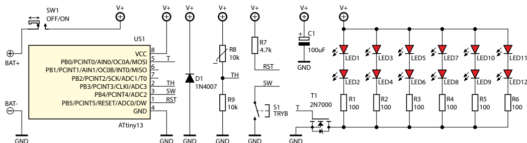
Figure 1. Schematic diagram
