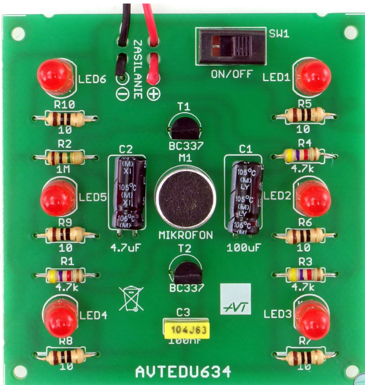
Photo 1. View of the assembled circuit board (Click to view)
