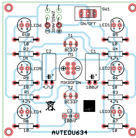
Figure 2. Position of the elements on the circuit board
