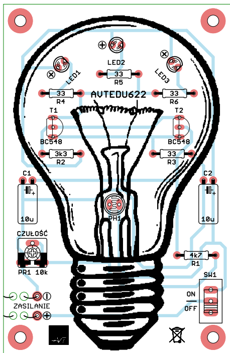
Figure 2. Position of the elements on the circuit board
